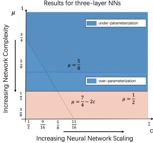
Figure 2: Scaling parameter c versus Network complexity parameter \mu for Part (a) in Corollary 8. Blue Region without dots : values of c and \mu where over-parameterization is necessary to achieve error bound \mathcal{O}(1/\sqrt{n}) . Blue Region with dots : values of c and \mu where under-parameterization is sufficient to achieve error bound \mathcal{O}(1/\sqrt{n}) . Pink Region : the desired bound cannot be guaranteed.
