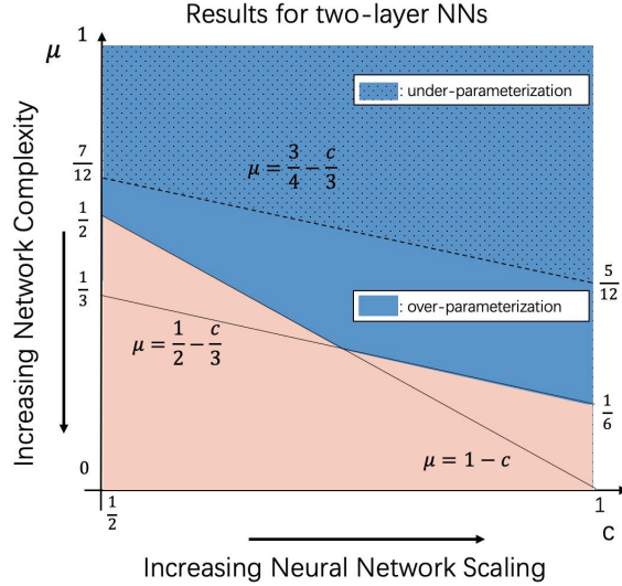
Figure 1: Scaling parameter c versus Network complexity parameter \mu for Part (a) in Corollary 4. Blue Region without dots : values of c and \mu where over-parameterization is necessary to achieve error bound \mathcal{O}(1/\sqrt{n}) . Blue Region with dots : values of c and \mu where under-parameterization is sufficient to achieve error bound \mathcal{O}(1/\sqrt{n}) . Pink Region : the desired bound cannot be guaranteed.
